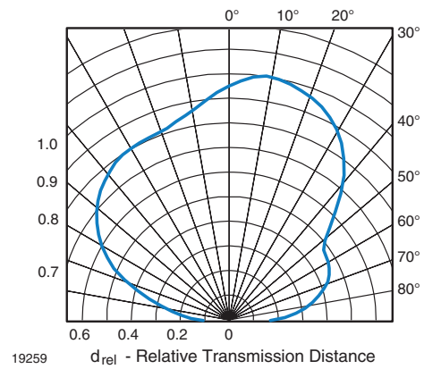
Fig. 4 - Vertical Directivity
