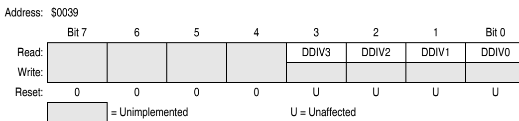
Figure 8-14. ICG DCO Divider Control Register (ICGDVR)
