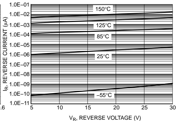
Figure 2. Reverse Leakage
