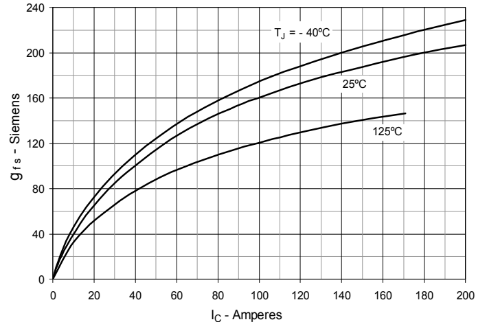
Fig. 6. Transconductance
