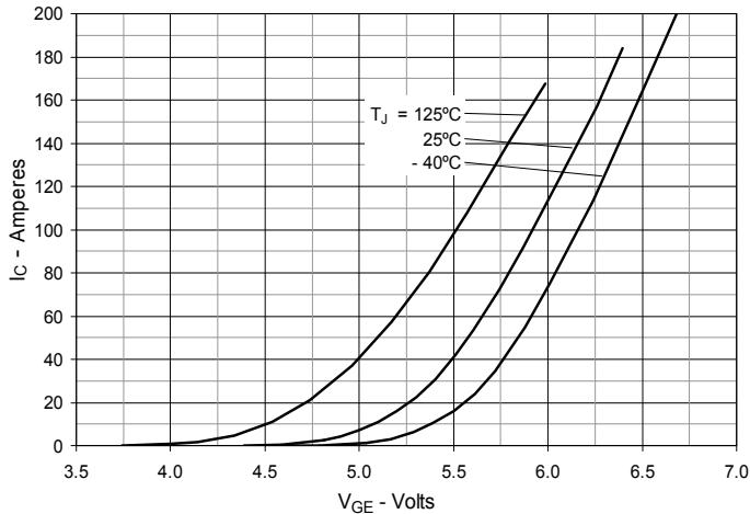
Fig. 5. Input Admittance
