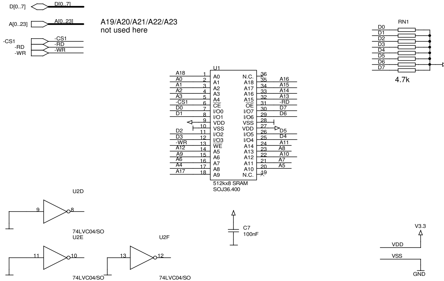
Figure 11. eZ80F92 Ethernet Module Schematic Diagram, #3 of 9—36-Pin SRAM Device
