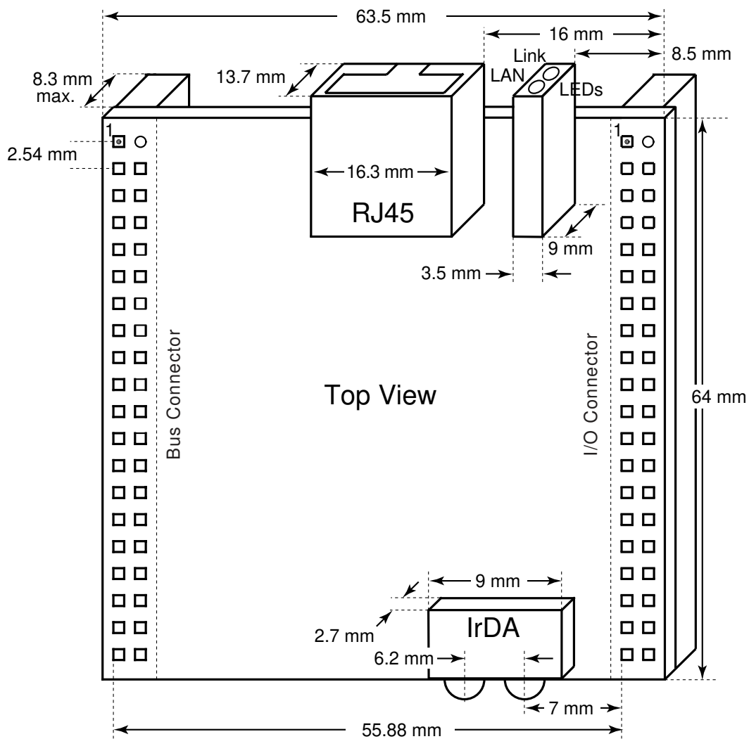
Figure 4. Dimension Drawing
