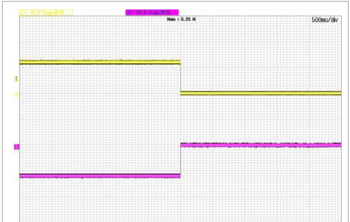
Shut-down enabled by disconnecting V_i at: T_{P1} = +25^\circ\text{C} , V_i = 24 V, I_o = +1.25 A resistive load. Top trace: output1 voltage (10 V/div.). Bottom trace: output2 voltage (10 V/div.). Time scale: (500 ms/div.).
