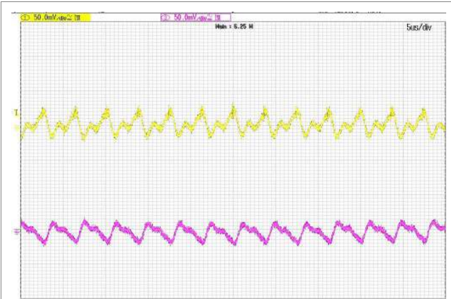
Output voltage ripple at: T_{P1} = +25^\circ\text{C} , V_I = 24 V, I_O = +1.0 A resistive load. Trace: output voltage (50 mV/div.). Time scale: (5 \mu\text{s} /div.). 20 MHz bandwidth
