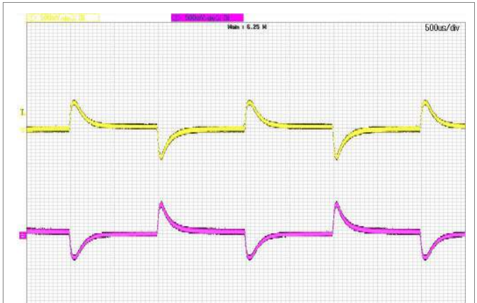
Output voltage response to load current step-change \pm(0.3125-0.625-0.3125 A) at: T_{P1} = +25^\circ\text{C} , V_i = 24 V. Top trace: output1 voltage (500 mV/div.). Bottom trace: output2 voltage (500 mV/div.). Time scale: (500 \mu\text{s} /div.).
