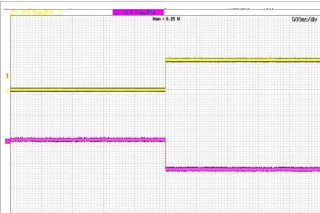
Start-up enabled by connecting V_i at: T_{P1} = +25^\circ\text{C} , V_i = 24 V, I_o = +1.25 A resistive load. Top trace: output1 voltage (10 V/div.). Bottom trace: output2 voltage (10 V/div.). Time scale: (500 ms/div.).
