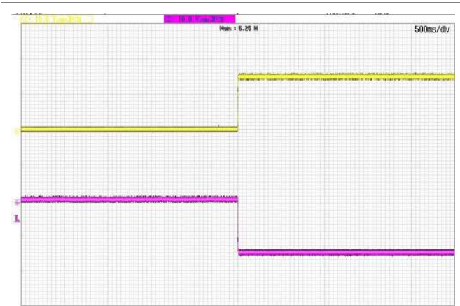
Start-up enabled by connecting V_I at: T_{P1} = +25^\circ\text{C} , V_I = 24 V, I_O = +1.0 A resistive load. Top trace: output1 voltage (10 V/div.). Bottom trace: output2 voltage (10 V/div.). Time scale: (500 ms/div.).
