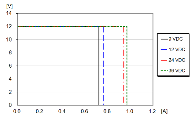
Output voltage vs. load current at I_o > \max I_o at +25°C. (Balance Load)
