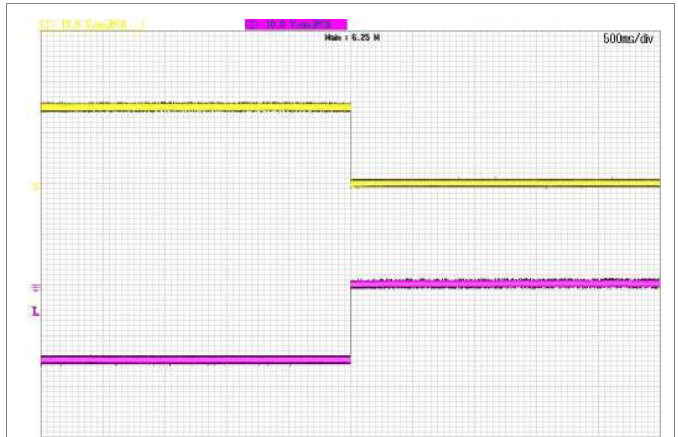
Shut-down enabled by disconnecting V_I at: T_{P1} = +25^\circ\text{C} , V_I = 24 V, I_O = +1.0 A resistive load. Top trace: output1 voltage (10 V/div.). Bottom trace: output2 voltage (10 V/div.). Time scale: (500 ms/div.).
