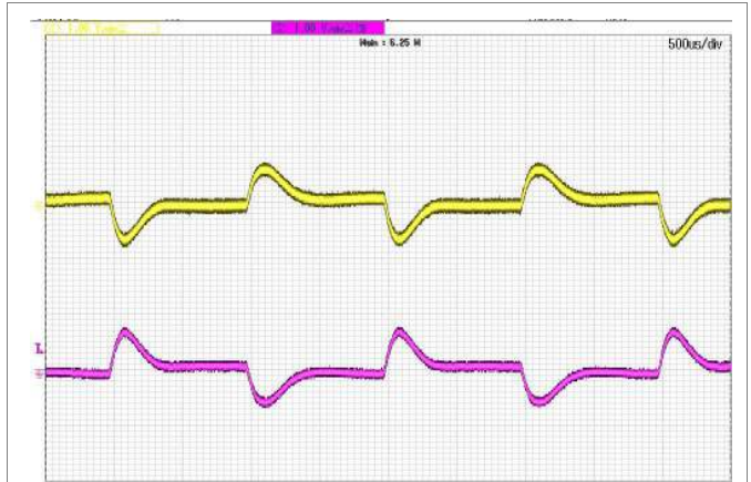
Output voltage response to load current step-change \pm(0.25-0.5-0.25 A) at: T_{P1} = +25^\circ\text{C} , V_I = 24 V. Top trace: output1 voltage (1 V/div.). Bottom trace: output2 voltage (1 V/div.). Time scale: (500 \mu\text{s} /div.).
