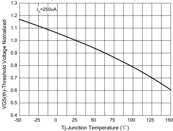
Fig. 5 - Normalized Threshold voltage
