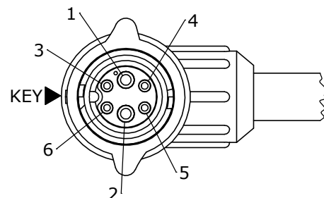
END "A" FACE VIEW
