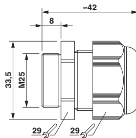
Dimensional drawing
