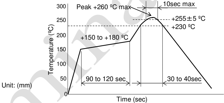
Fig.5 Reflow profile (Lead Free Available)
