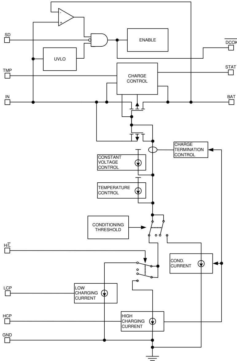
Figure 2 – Simplified Block Diagram
