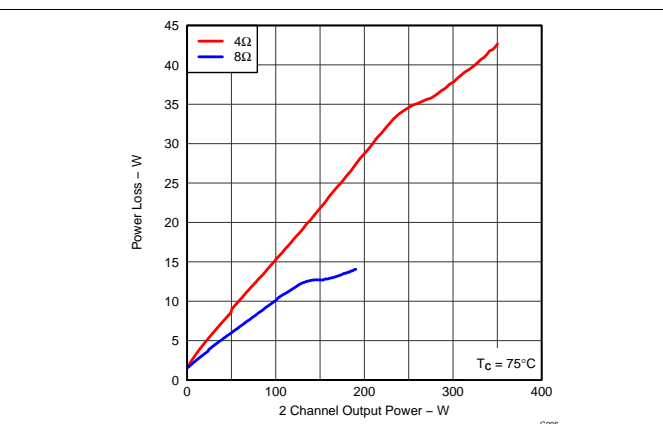
Figure 6. System Power Loss vs Output Power
