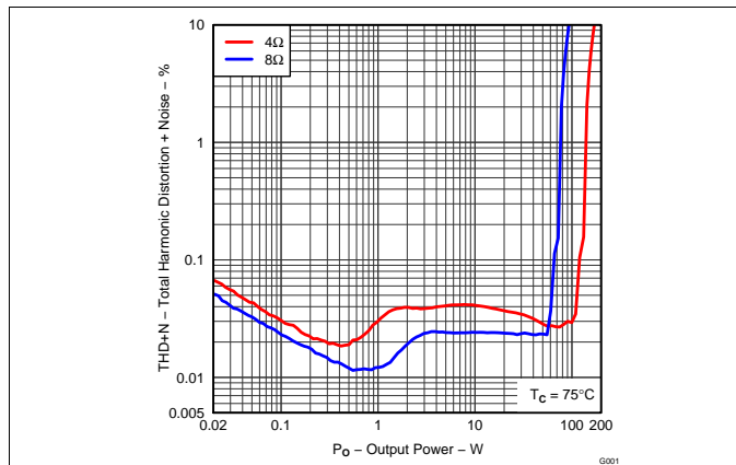
Figure 1. Total Harmonic + Noise vs Output Power, 1 kHz
