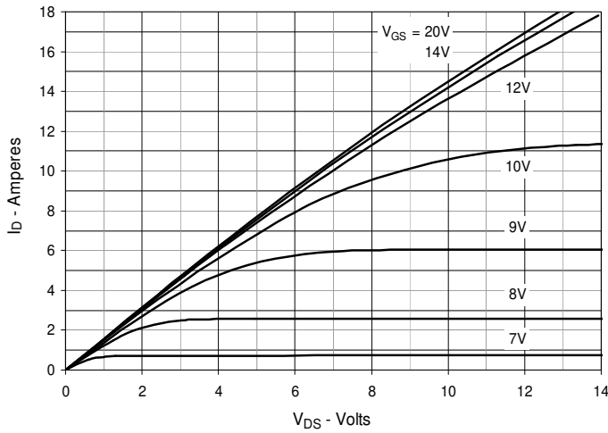
Fig. 1. Output Characteristics @ T J = 25°C
