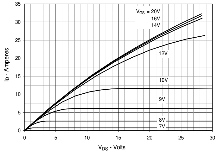
Fig. 2. Extended Output Characteristics @ T J = 25°C
