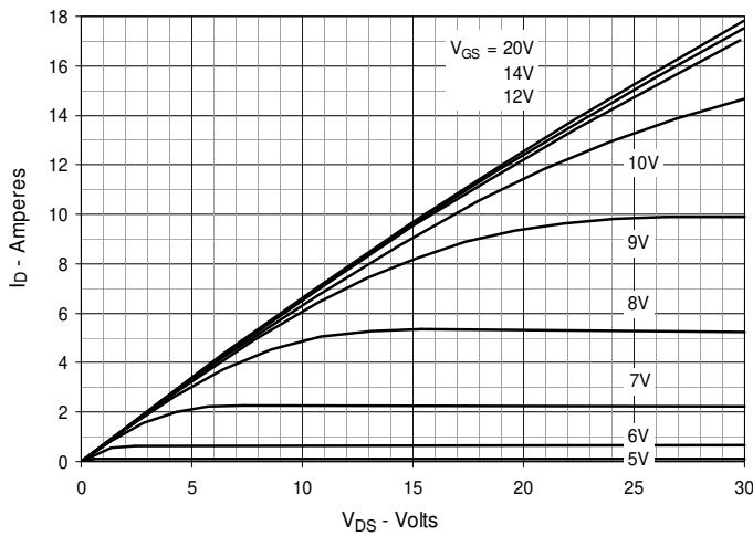
Fig. 3. Output Characteristics @ T J = 125°C
