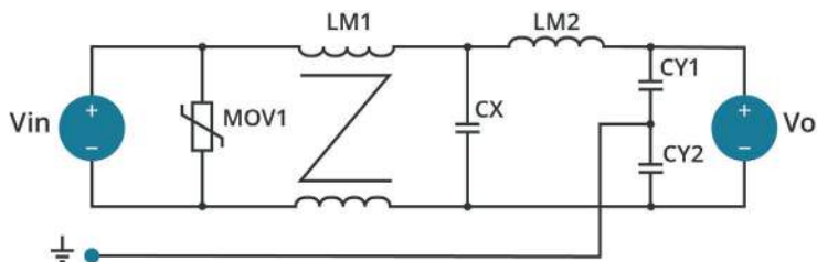
Figure 1 Internal Circuit
