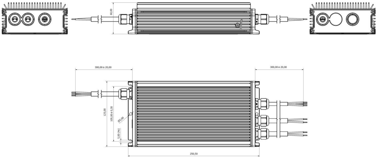
Figure 3. Mechanical drawing
