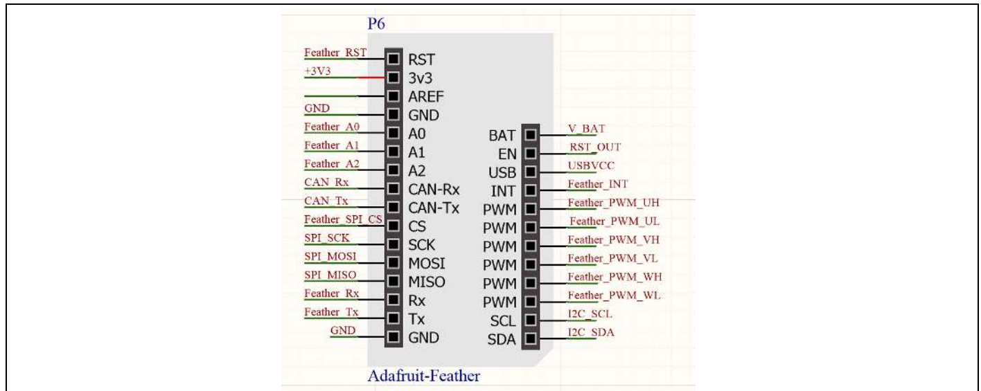
Figure 8 Adafuit Feather Wing™ pin assignments
