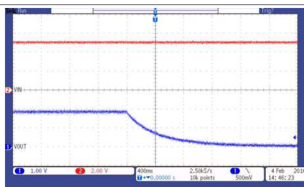
Figure 34. TPS737xx-Q1 Shutdown
