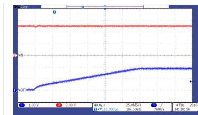
Figure 33. TPS737xx-Q1 Start-Up
