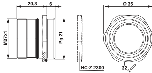
Dimensioned drawing
