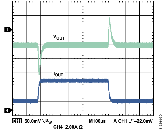
Figure 25. Channel 1/Channel 2 Load Transient, 1 A to 4 A, V_{IN} = 12\text{ V} , V_{OUT} = 3.3\text{ V} , f_{SW} = 600\text{ kHz} , L = 2.2\text{ }\mu\text{H} , C_{OUT} = 47\text{ }\mu\text{F} \times 2
