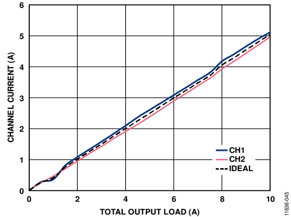
Figure 40. Current Balance in Parallel Output Configuration, V IN = 12 V, V OUT = 1.2 V, f sw = 600 kHz, FPWM Mode
