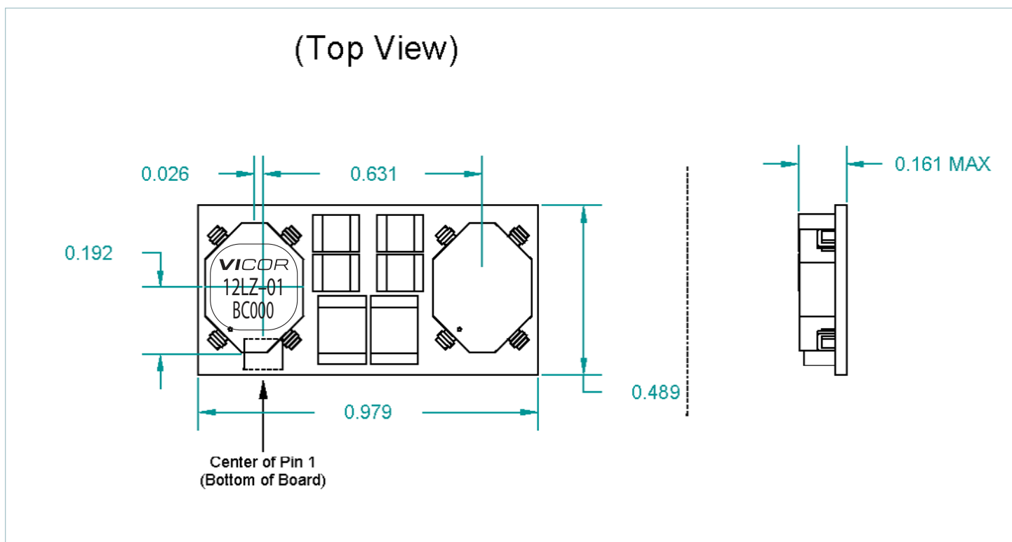
Figure 19 — Open-frame package dimensions, tolerance of \pm 0.004in ; pick-and-place from label center
