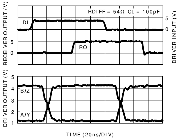
FIGURE 20. DRIVER AND RECEIVER WAVEFORMS, (I SL3156E, I SL3158E)
