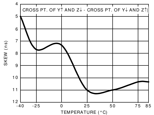
FIGURE 13. DRIVER DIFFERENTIAL SKEW vs TEMPERATURE (I SL3150E, I SL3152E)
