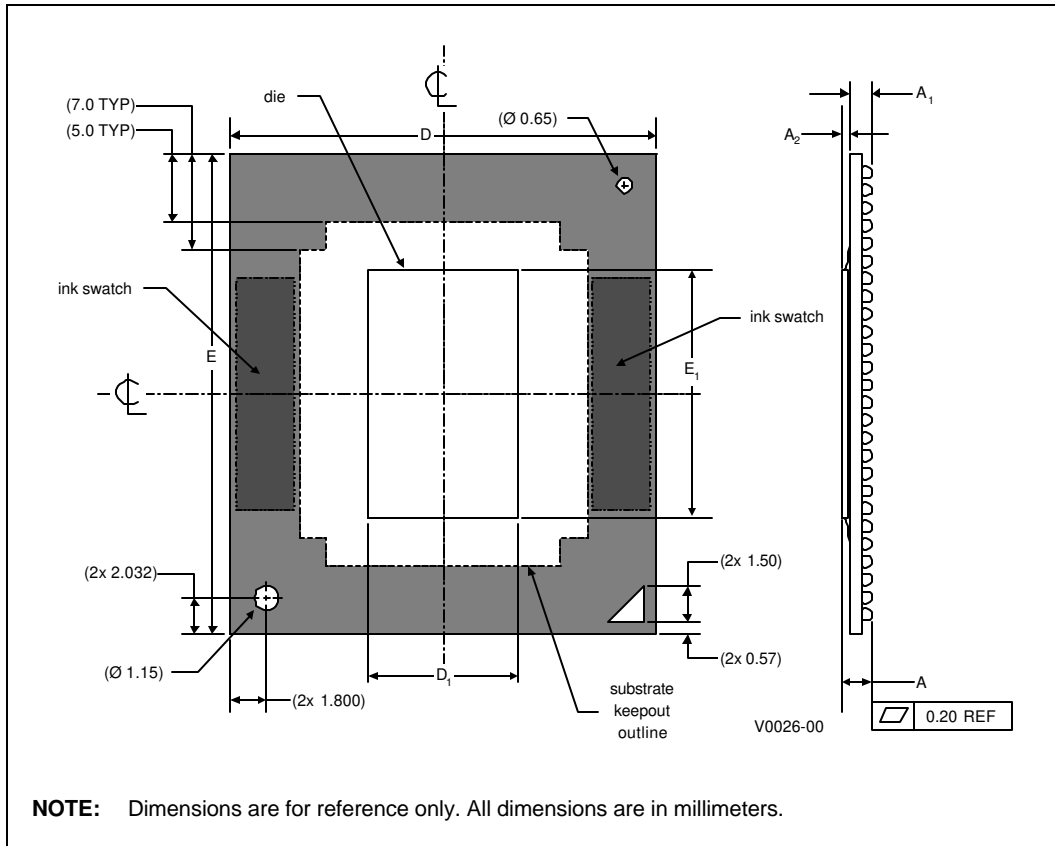
Figure 5.3 Surface-mount BGA Package - Top and Side View
