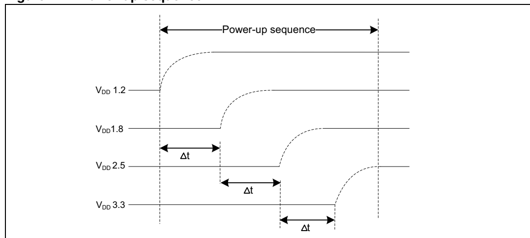
Figure 4. Power-up sequence
