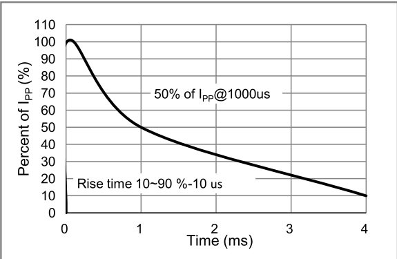
Fig.3 10/1000us Pulse Waveform
