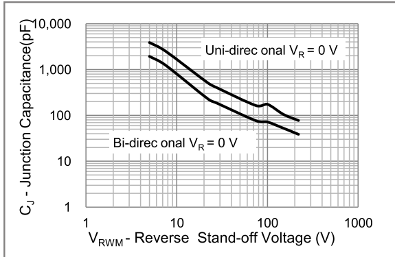
Fig.4 Typical Capacitance
