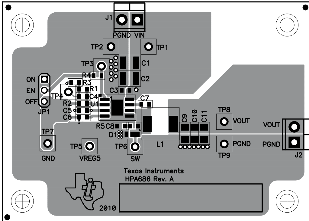
Figure 5-1. Top Assembly
