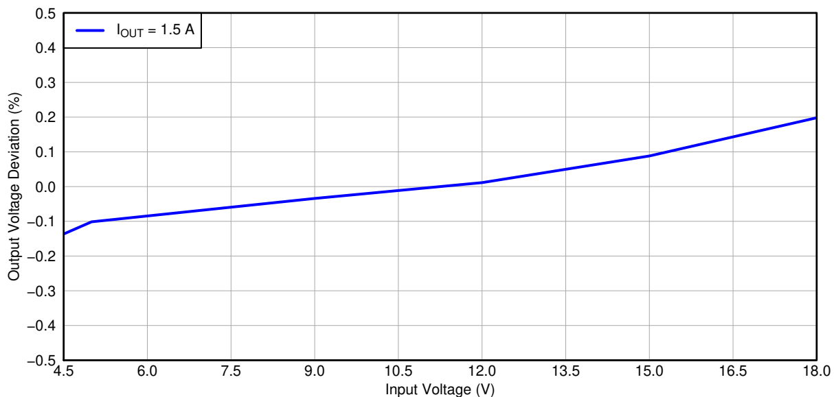
Figure 4-5. TPS54327EVM-686 Line Regulation
