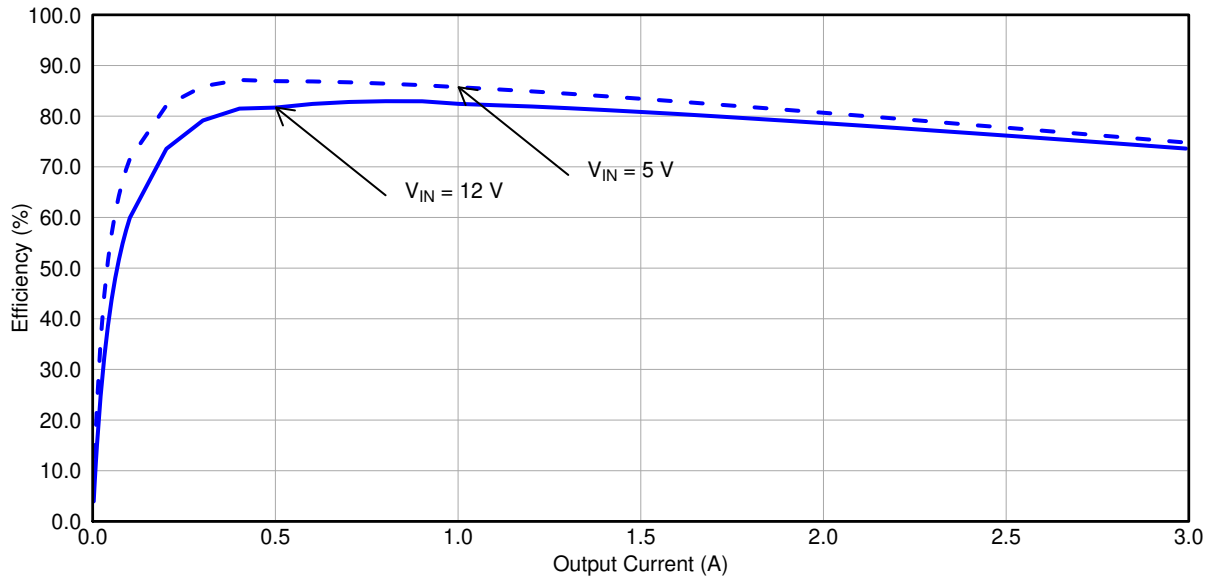
Figure 4-1. TPS54327EVM-686 Efficiency
