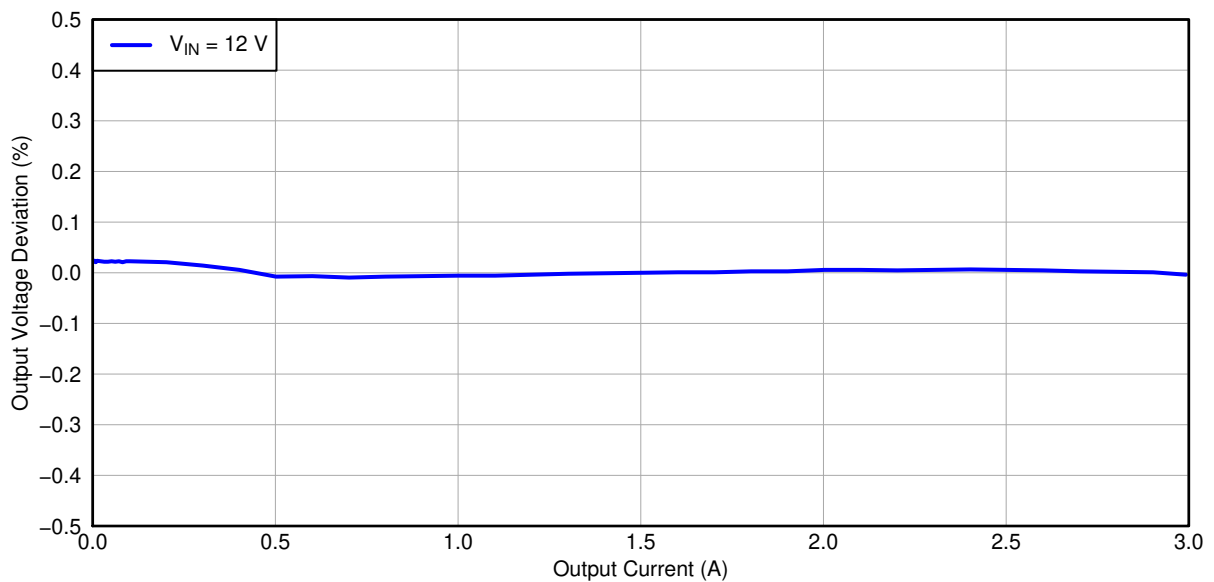
Figure 4-4. TPS54327EVM-686 Load Regulation, V_{IN} = 12\text{ V} .
