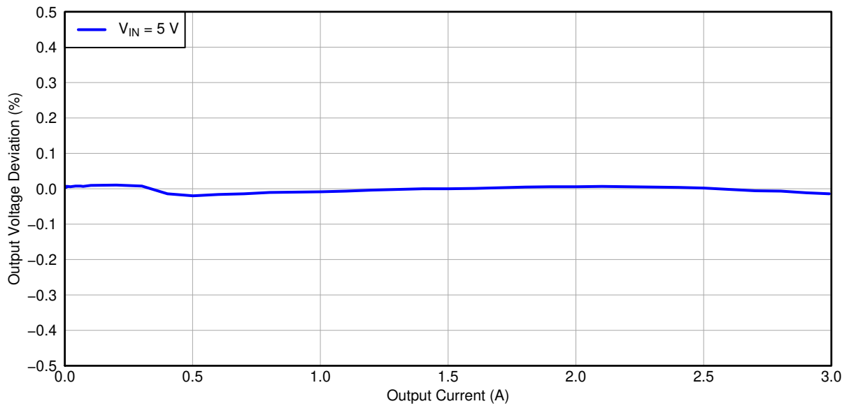
Figure 4-3. TPS54327EVM-686 Load Regulation, V_{IN} = 5\text{ V} .
