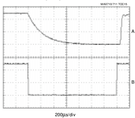
TURN-OFF DELAY
