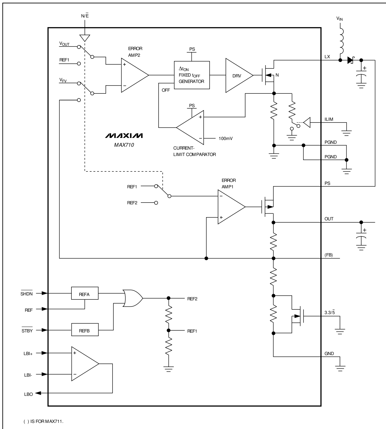
Figure 1. Functional Diagram
