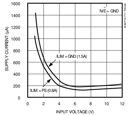
NO-LOAD BATTERY CURRENT vs. INPUT VOLTAGE
