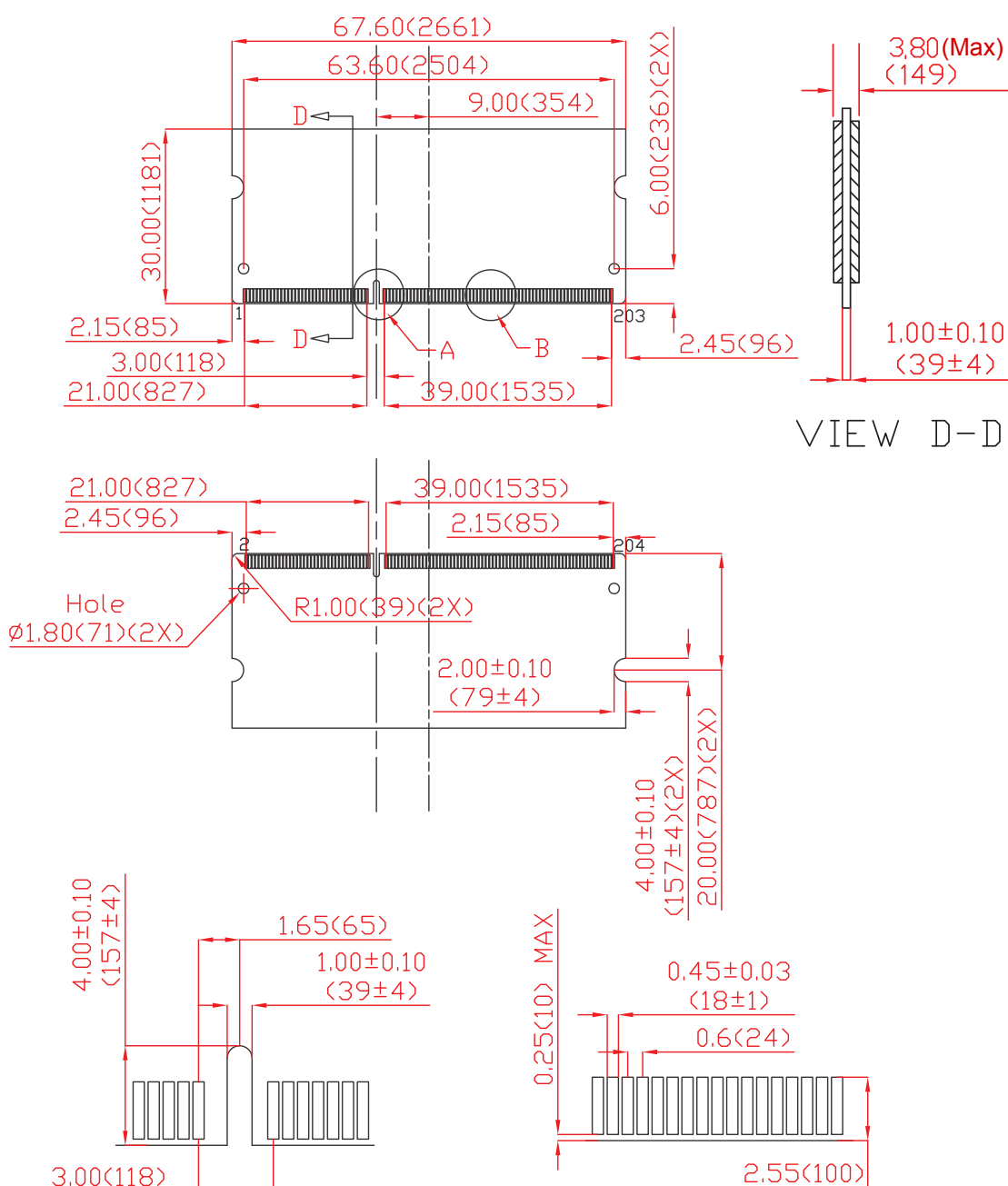
Detail A
