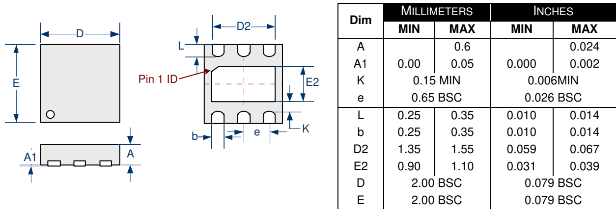
Figure 13 · LU 6-Pin Plastic UDFN 2mm x 2mm x 0.6mm Package Dimensions
