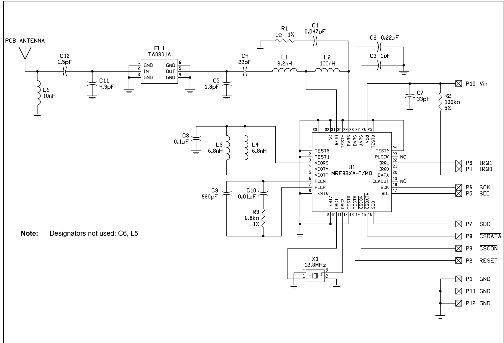
FIGURE 2-2: MRF89XAM8A SCHEMATIC
