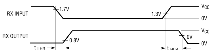
Receiver Propagation Delay Timing
