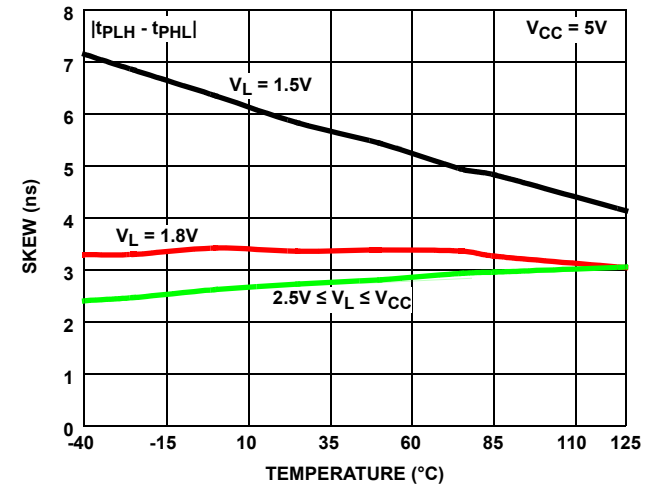
FIGURE 25. ISL3227xE RECEIVER SKEW vs TEMPERATURE
