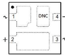
Top View Pin Configuration **Do Not Connect the DNC Pad**
