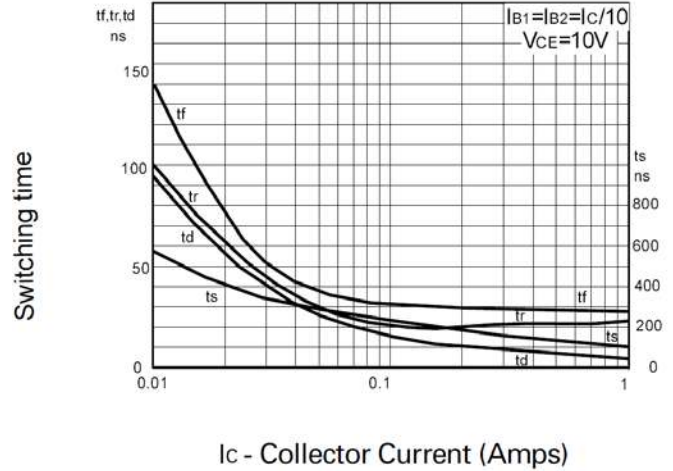
Switching Speeds
