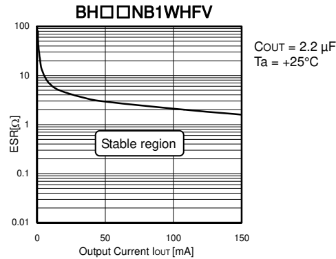
Fig.30 Stable Operation Region (Example)
