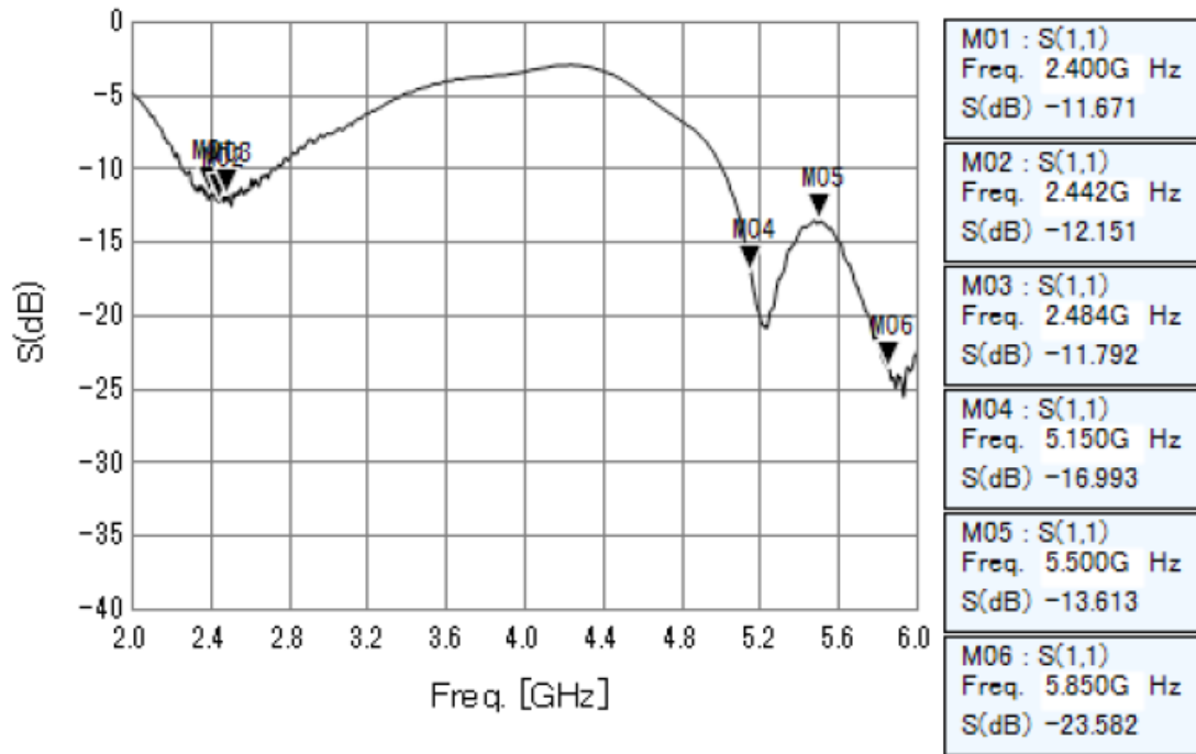
Figure 13 – Return Loss for 1LV M.2 Module Standalone
