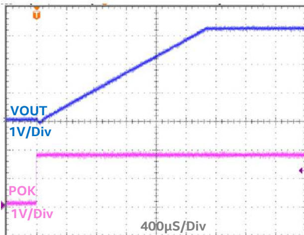
Start-up: V_{IN} = 5.0V , V_{OUT} = 3.3V
