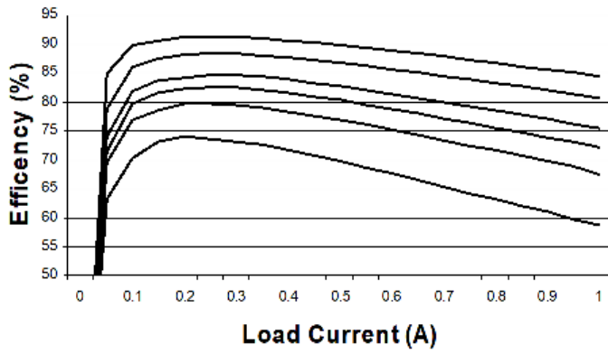
Efficiency Vs. Load Current ( V_{in} = 5.0V )
