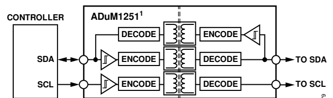
1 ADDITIONAL PINS OMITTED FOR CLARITY.
