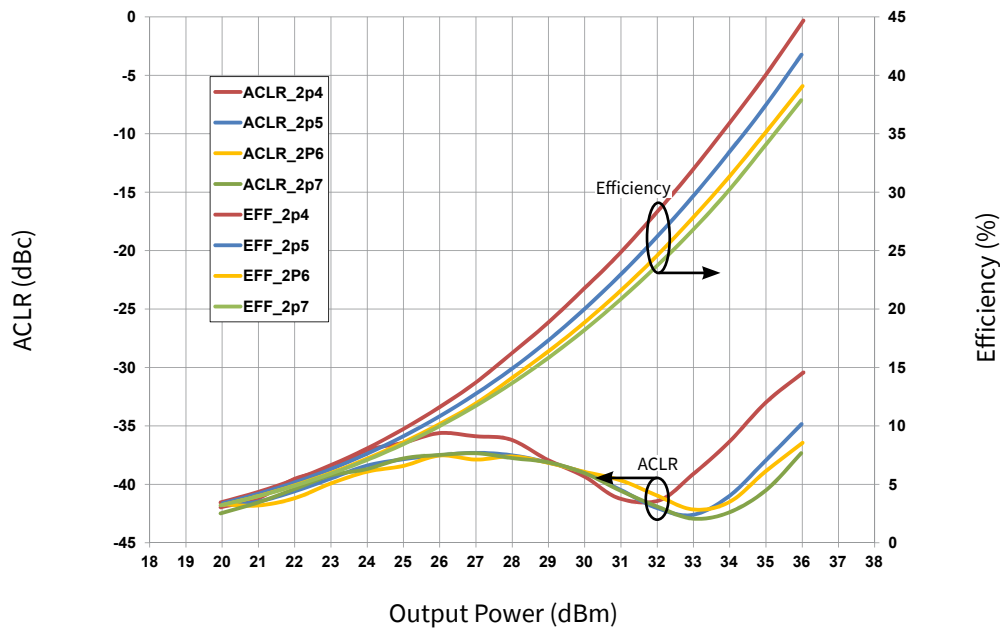
Figure 2. Typical Drain Efficiency and ACLR vs. Output Power V_{DD} = 50\text{ V}, I_{DQ} = 60\text{ mA}, 1\text{ Carrier WCDMA}, \text{PAR} = 7.5\text{ dB}
