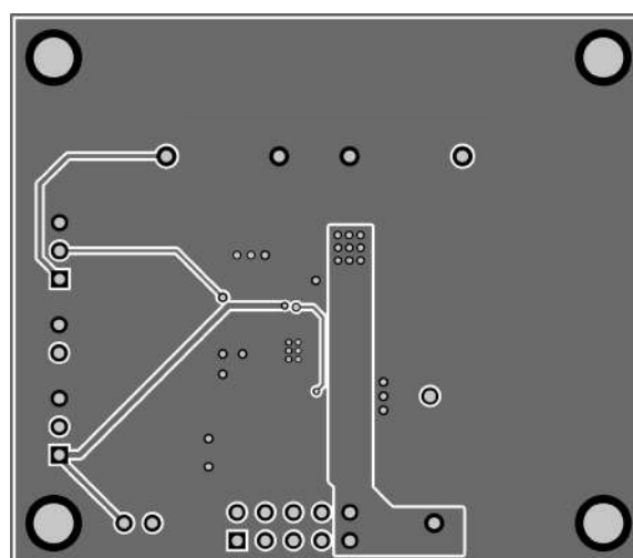
Figure 6: AAT1409IMK Evaluation Board Bottom Side Layout.
