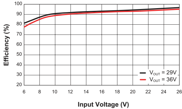
Boost Efficiency vs. Input Voltage ( L = 10\mu\text{H} ; V_{CC} = 4.7\text{V} ; \text{PWM} = V_{CC} ; F_{SET} = \text{GND} ; I_{OUT} = 360\text{mA} )
