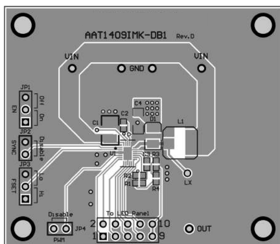
Figure 5: AAT1409IMK Evaluation Board Top Side Layout.
