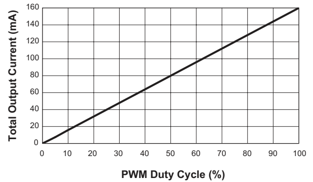
Output Current vs. PWM Duty Cycle ( V_{IN} = 12\text{V} ; I_{CSx} = 20\text{mA/ch} )
