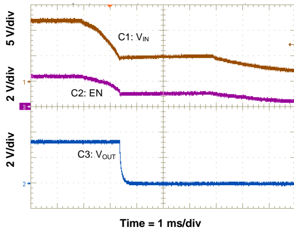
Figure 19. Shutdown Relative to V_{IN}
