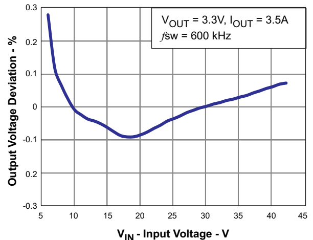
Figure 7. Regulation Versus Input Voltage
