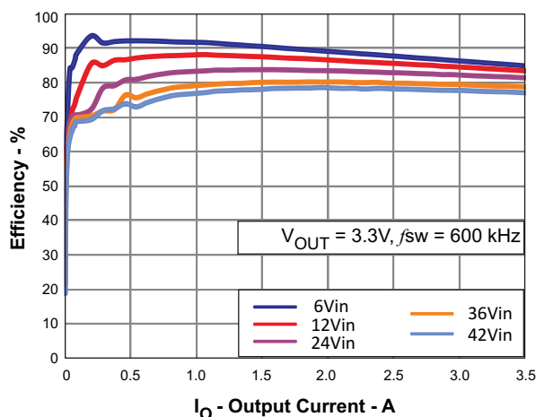
Figure 2. Efficiency Versus Load Current
