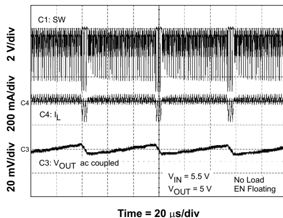
Figure 21. Low Dropout Operation
