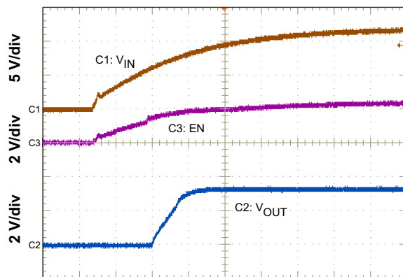
Time = 2 ms/div Figure 16. Start Up Relative to V_{IN}
