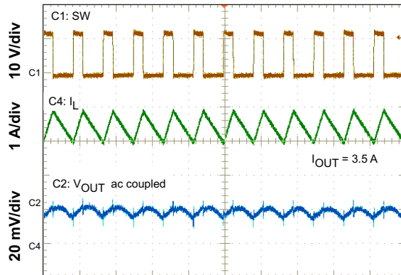
Time = 2 \mu s/div Figure 11. Output Voltage Ripple CCM
