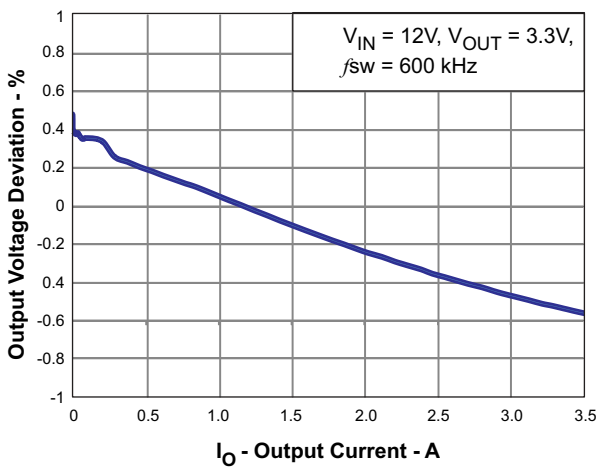
Figure 6. Regulation Versus Output Current
