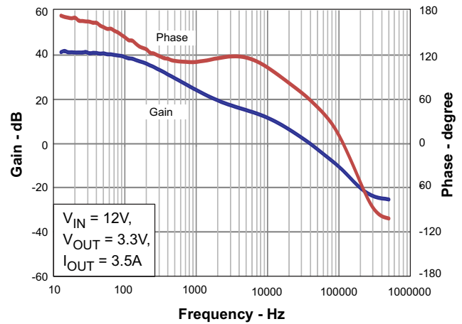
Figure 9. Loop Response
