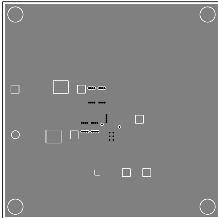
Figure 25. TPS54340EVM-182 Layer 2 Layout
