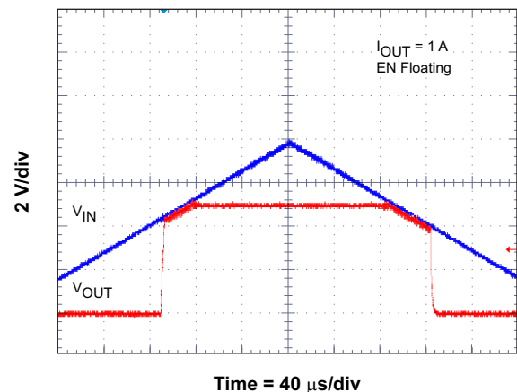
Figure 22. Low Dropout Start Up and Shutdown
