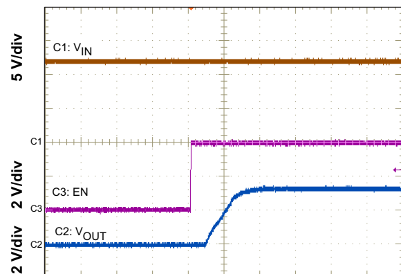
Time = 2 ms/div Figure 17. Start Up Relative to EN
