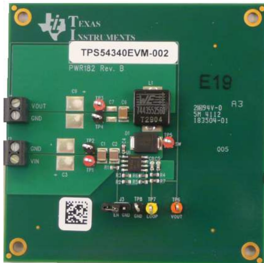
Figure 1. TPS54340EVM-182 Board
