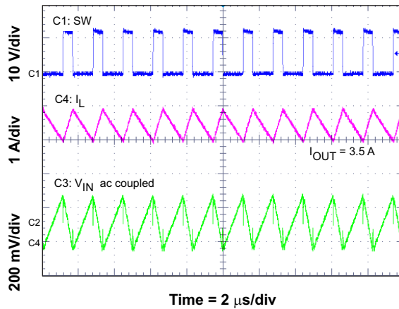
Figure 14. Input Voltage Ripple CCM
