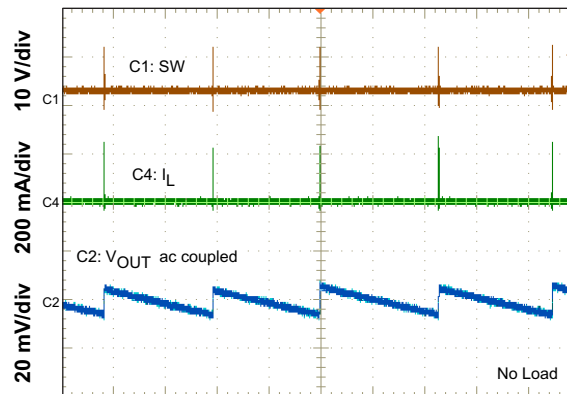
Time = 2 ms/div Figure 13. Output Voltage Ripple Eco-mode
