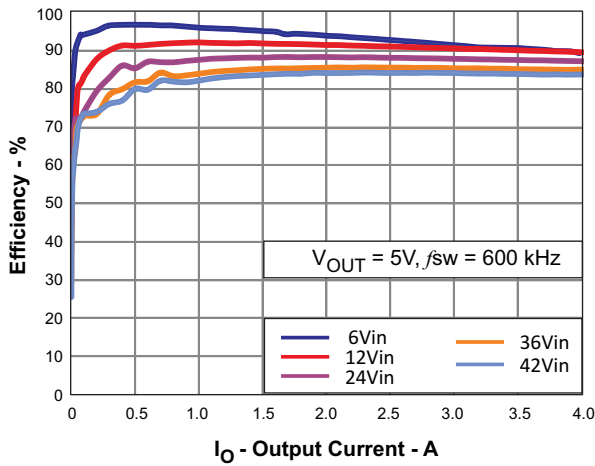
Figure 4. Efficiency Versus Load Current
