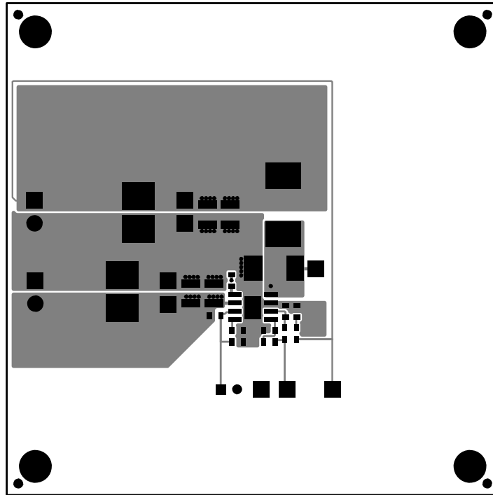
Figure 24. TPS54340EVM-182 Top-Side Layout
