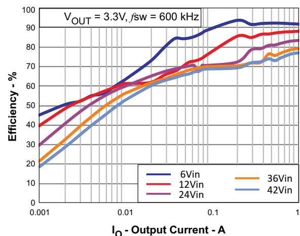
Figure 3. Light-Load Efficiency
