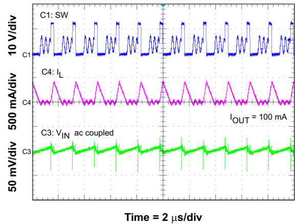
Figure 15. Input Voltage Ripple DCM
