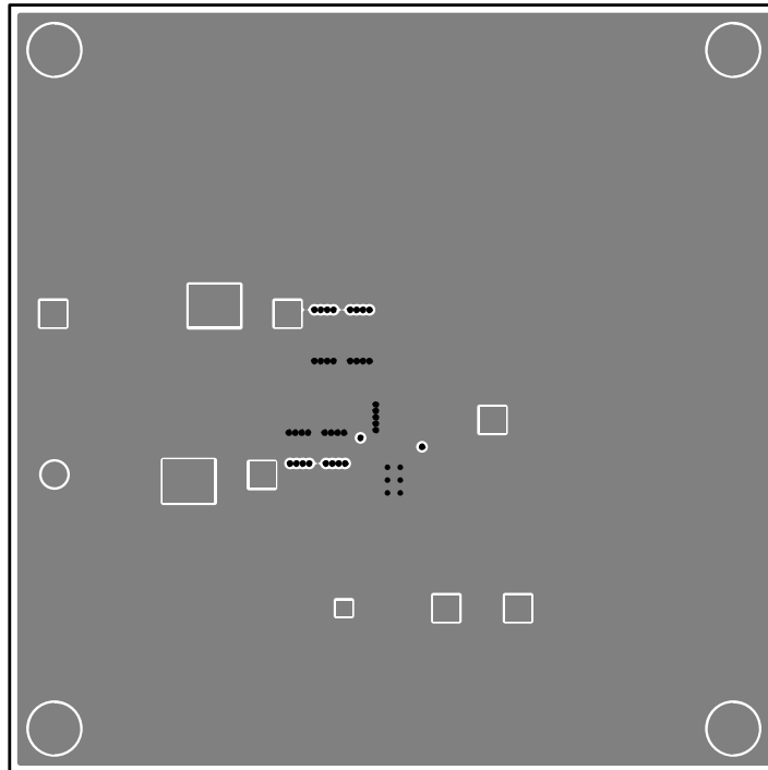
Figure 26. TPS54340EVM-182 Layer 3 Layout
