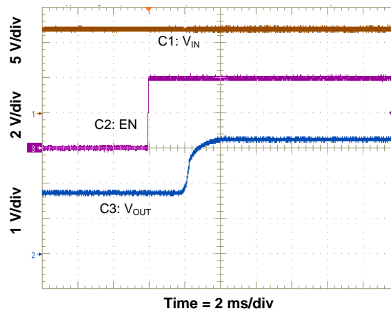
Time = 2 ms/div Figure 18. Prebias Start Up Relative to EN
