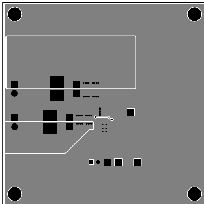
Figure 27. TPS54340EVM-182 Bottom-Side Layout
