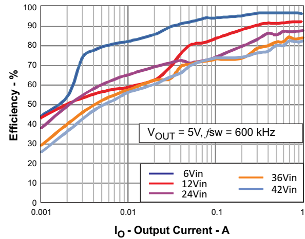
Figure 5. Light Load Efficiency
