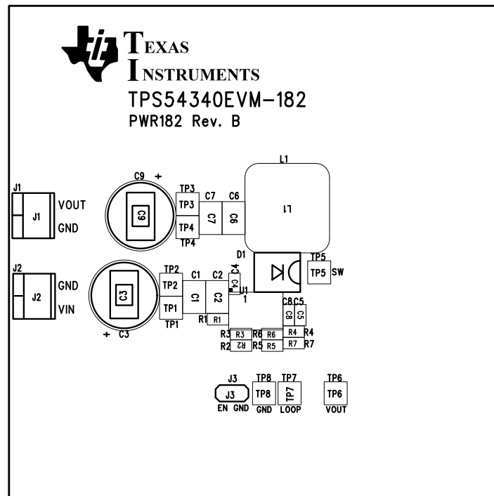
Figure 23. TPS54340EVM-182 Top Assembly and Silkscreen
