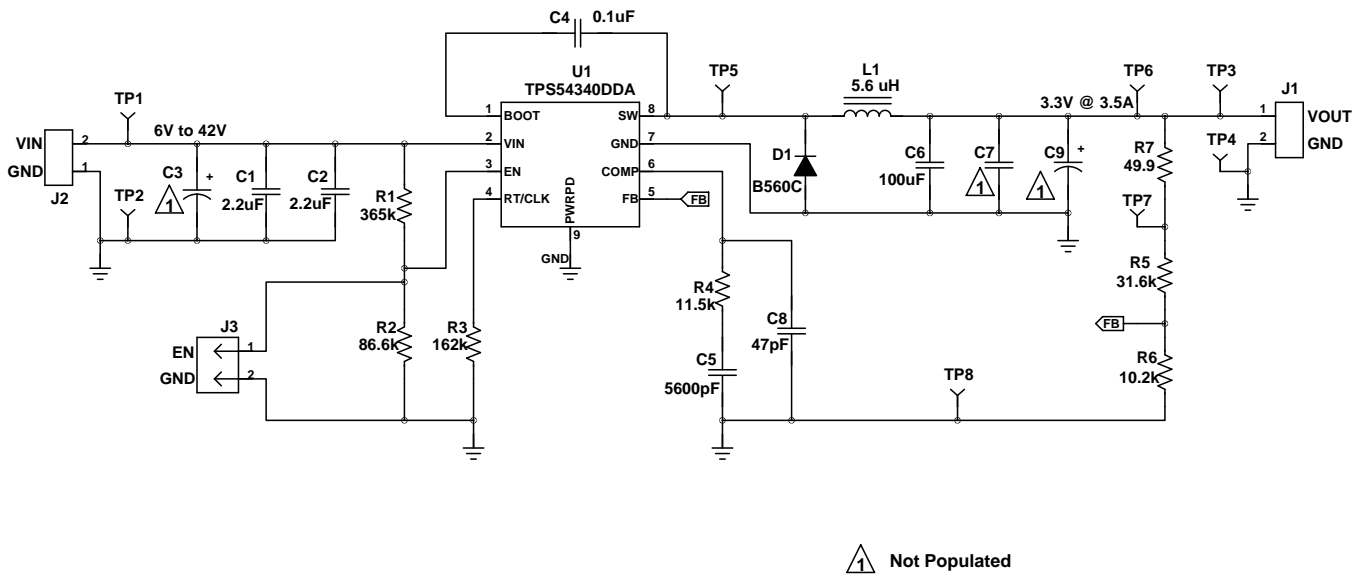
Figure 28. TPS54340EVM-182 Schematic
