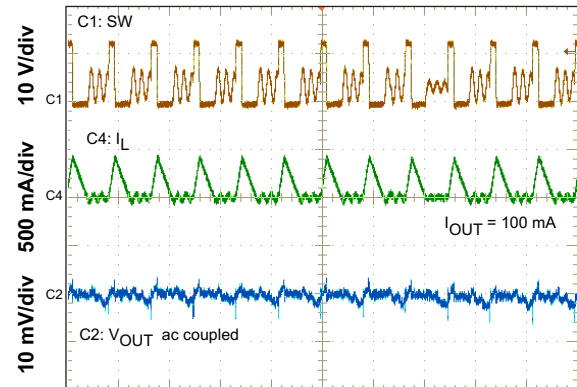
Time = 2 \mu s/div Figure 12. Output Voltage Ripple DCM
