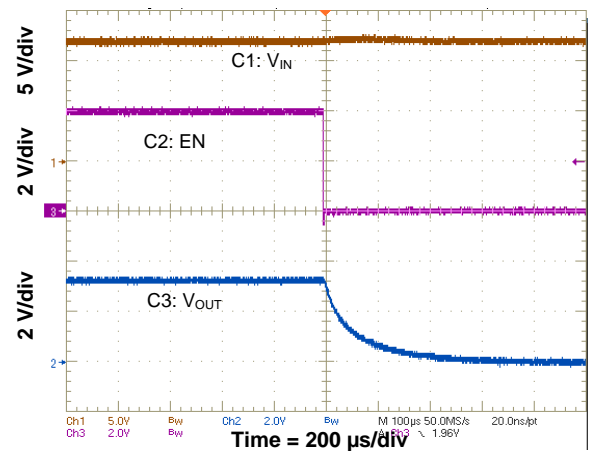
Figure 20. Shutdown Relative to EN
