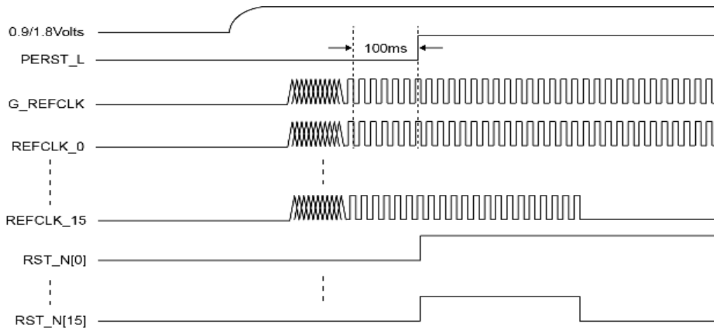
Figure 6-1 Timing Sequence for Surprised Hot Plug Operation
