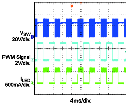
PWM Dimming
