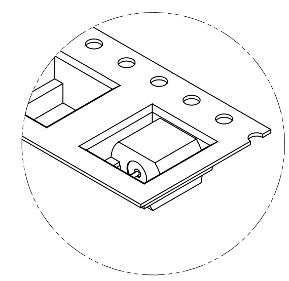
DETAIL C SCALE 3:1
