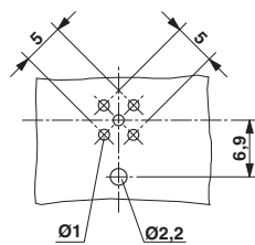
Drilling diagram
