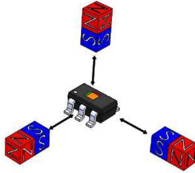
Figure 8-4. Axis Polarities
