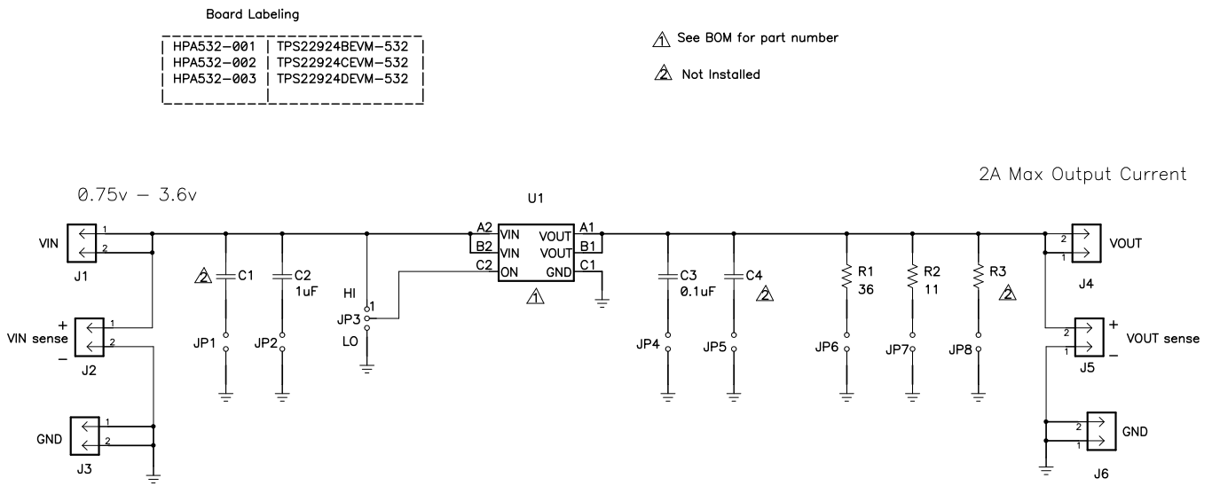
Figure 5. TPS22924EVM-532 Schematic
