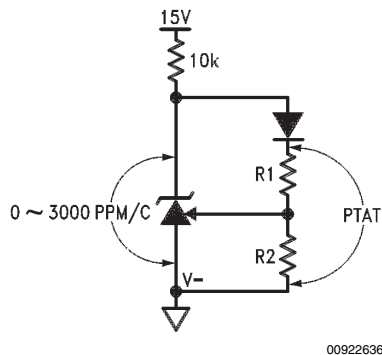
FIGURE 8. Diode in Series with R1 Causes Voltage Across R1 and R2 to be Proportional to Absolute Temperature (PTAT)
