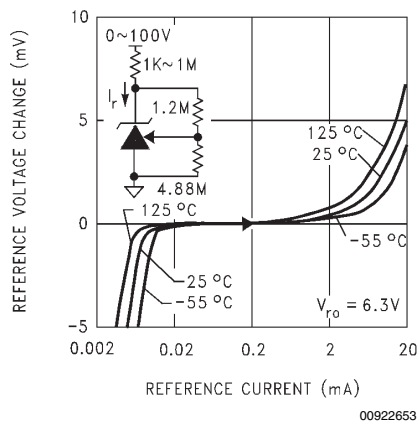
Reference Voltage vs Current and Temperature
