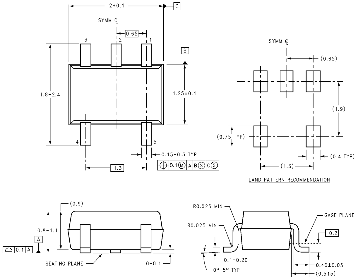
5-Pin SC70-5 NSC Package Number MAA05A
