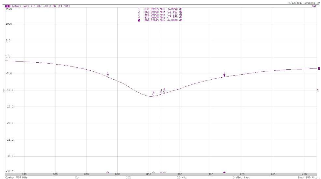
Figure 4: Typical antenna reflection performance
