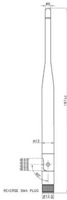
Figure 1: Physical dimensions
