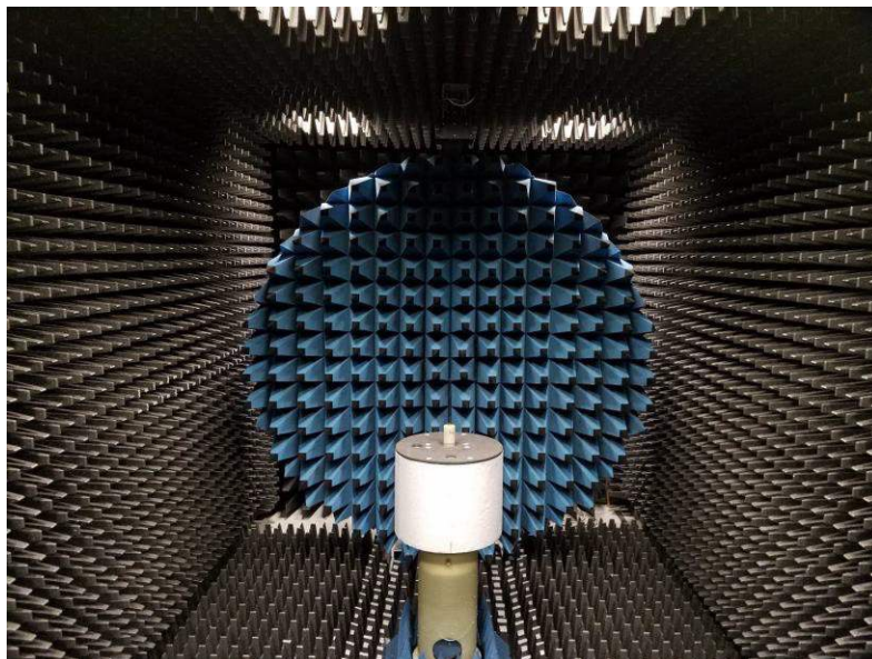
Figure 2: Antenna chamber
