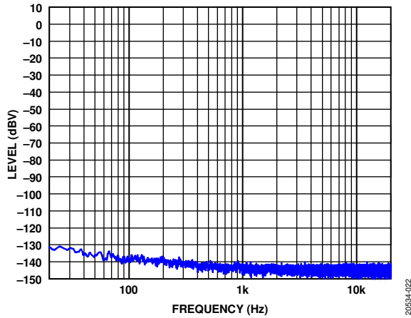
Figure 21. FFT, No Signal, f_s = 48 kHz, Signal Path = SDATA1_0 to HPOUTx0, Headphone Mode, Load = 16 \Omega
