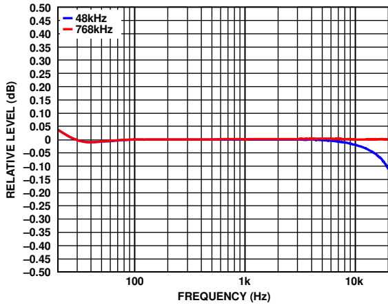
Figure 45. Relative Level vs. Frequency, Headphone/Line Output Mode, Load = 16 Ω to 10 kΩ, f_s = 48 kHz and 768 kHz, Signal Path = AIN0 to DAC0
