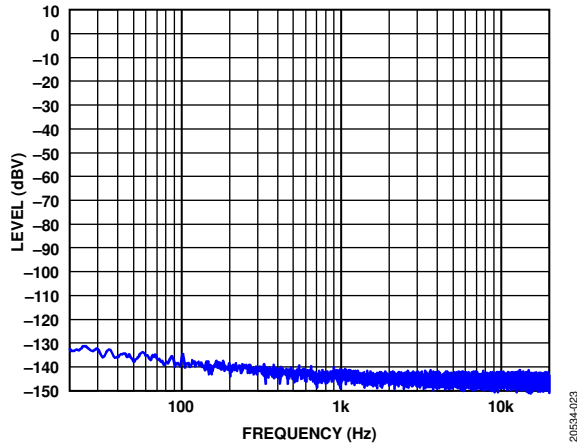
Figure 22. FFT, No Signal, f_s = 48 kHz, Signal Path = SDATA1_0 to LOUTx0, Line Output Mode, Load = 10 \text{ k}\Omega
