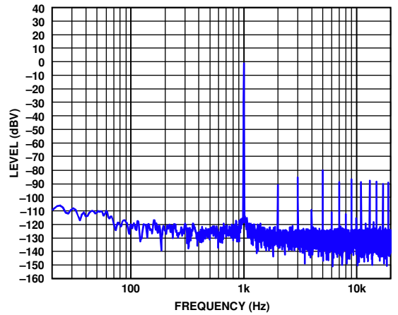
Figure 48. FFT, -1 dBV, Headphone Mode, Load = 16 Ω, f_s = 48 kHz to 768 kHz, Signal Path = AINx to HPOUTx0
