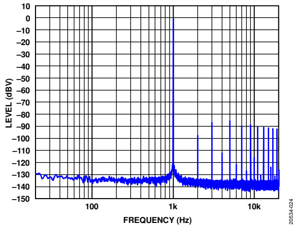
Figure 23. FFT, -1 dBFS, f_s = 48 kHz, Signal Path = SDATA1_0 to HPOUTx0, Headphone Mode, Load = 32 \Omega
